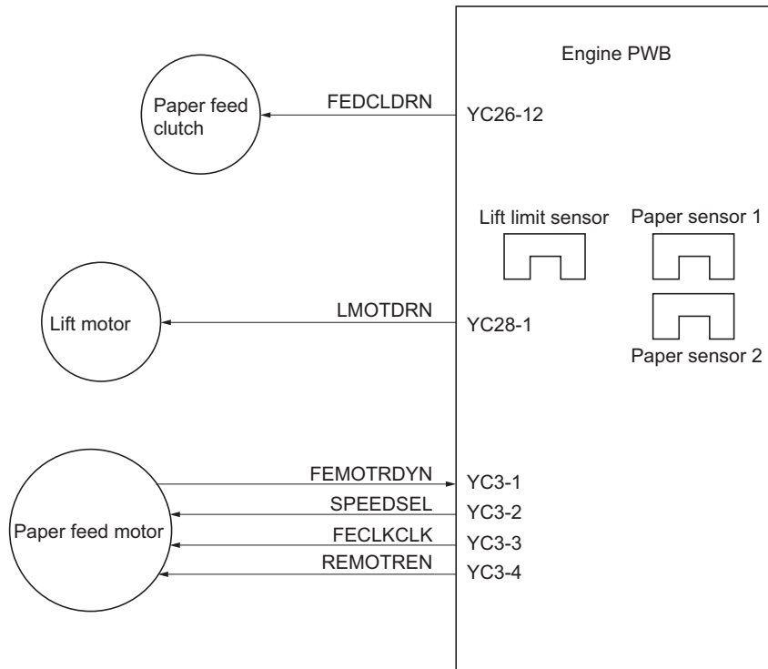
Figure 2-1-2Cassette paper feed section block diagram
