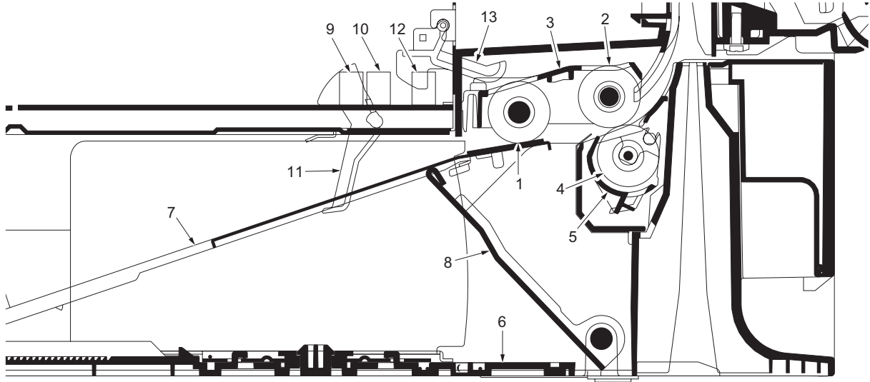
Figure 2-1-1 Cassette paper feed section
