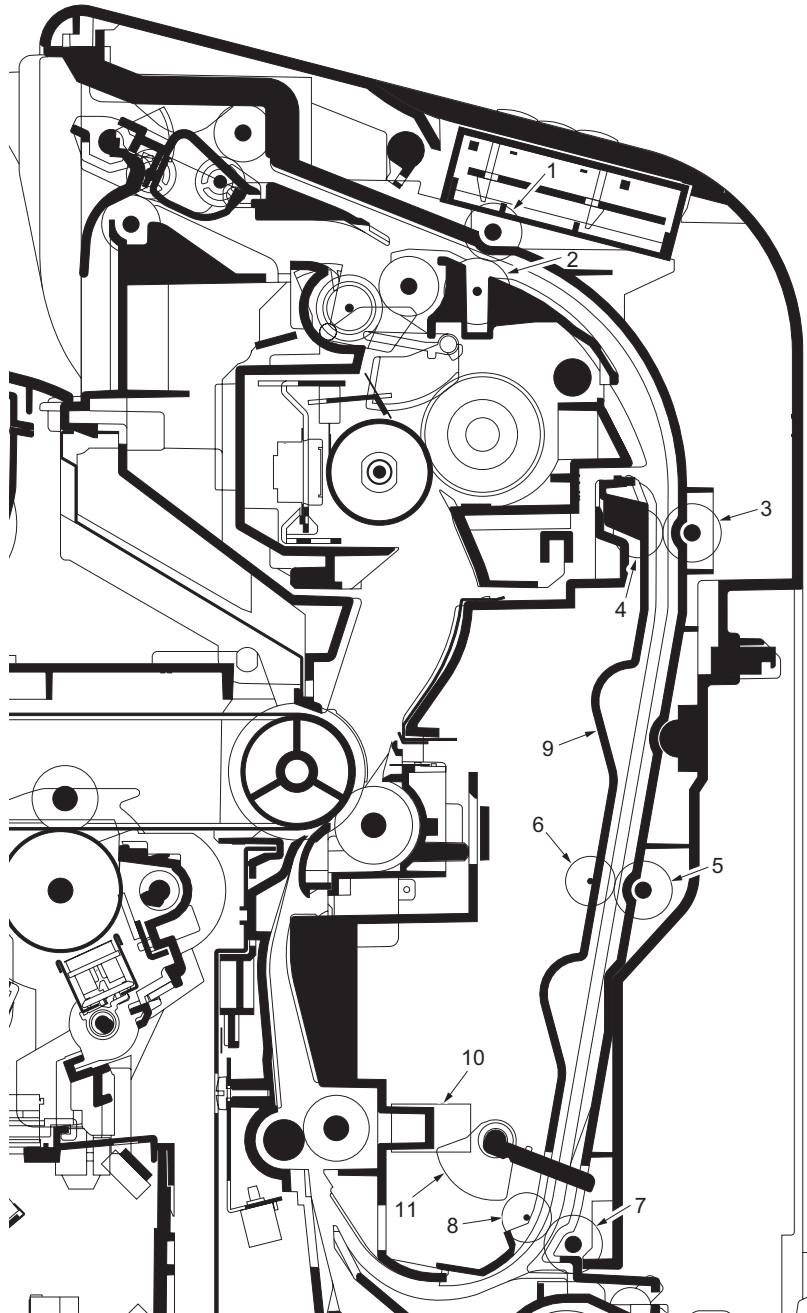
Figure 2-1-22 Duplex/conveying section
