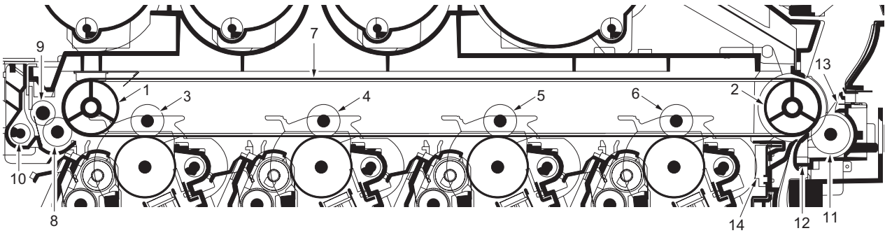
Figure 2-1-16 Transfer/separation section
